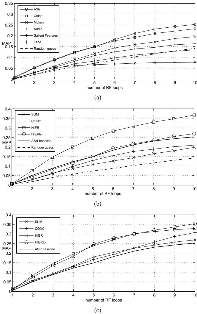
Fig. 13. TRECVID 05 Search Task: a) Relevance feedback simulation for every modality, b) when fusing 6 modalities and c) when fusing only the 4 best modalities (ASR, Color, Motion and Audio). At each iteration, up to 10 positive and negative examples are added to the query. SVM with automatic scale setting is used (where appropriate).
