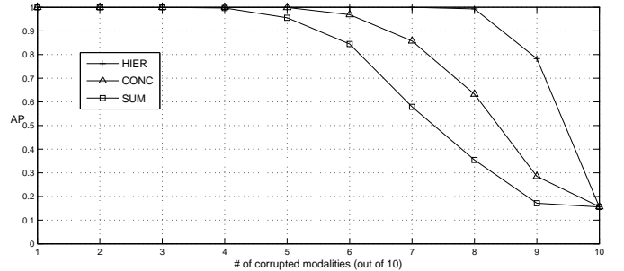
Fig. 12. Artificial data: Effect of corrupted modalities on the retrieval performance.
