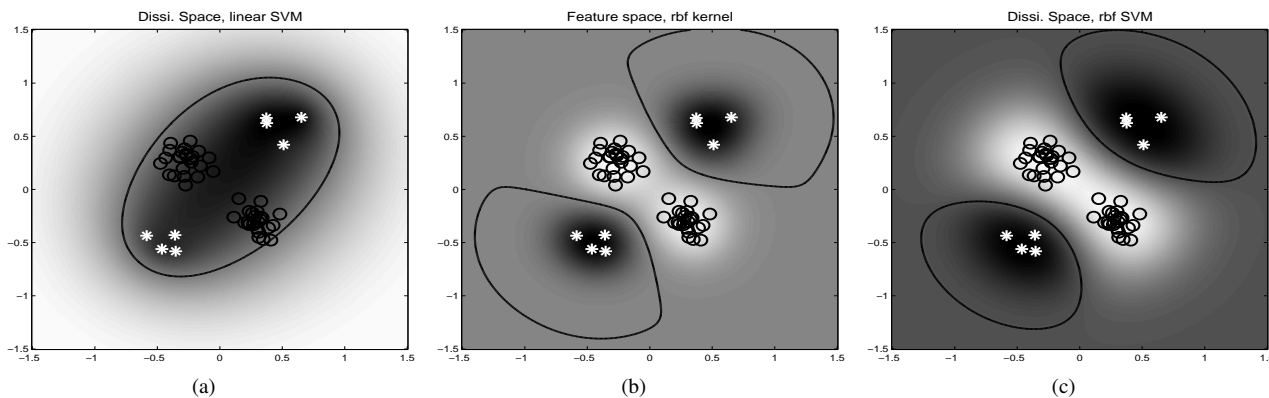
Fig. 4. Toy example: Decision function for the XOR configuration in 2D feature space. Circles are negative examples, stars are the positive samples. The gray level indicates relevance to the positive class (black = relevant, white = irrelevant). Black line indicates the separating hyperplane.
