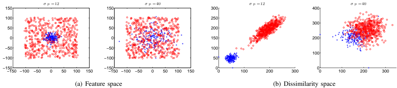
Fig. 5. Artificial data: Blue crosses represent positive elements drawn from \mathcal{N}(0, \sigma_P) , while red circles represent the negative samples uniformly distributed around the center of the space.
