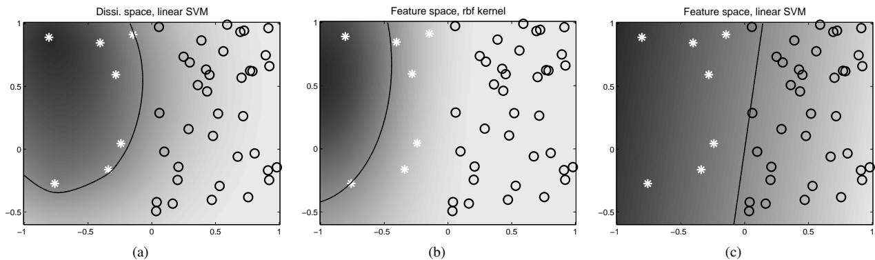
Fig. 3. Toy example: Decision function for the linear configuration in 2D feature space. Circles are negative examples, stars are the positive samples. The gray level indicates relevance to the positive class (black = relevant, white = irrelevant). Black line indicates the separating hyperplane.
