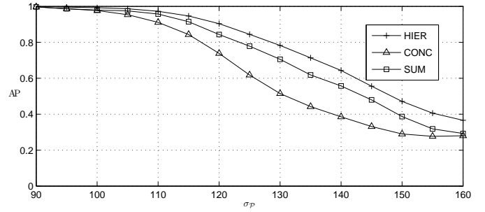
Fig. 11. Artificial data: Discriminating power with data less and less separable.
