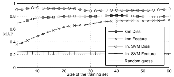
Fig. 6. Artificial data: Average precision for linear-SVM and k -NN in dissimilarity and feature space for a growing train set. A 10-dimension artificial space with \sigma_P = 80 is used.
